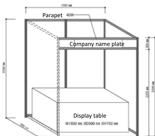
- Booth spec: Type A & C -
